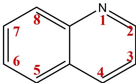
quinoline
