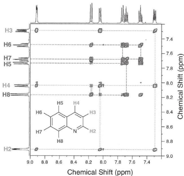
quinoline
